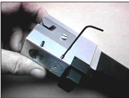
Figure 27. Removal of lower sealing plug
