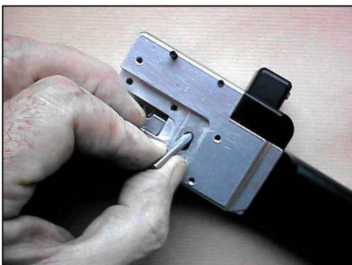
Figure 31. Remove knife drive shaft
