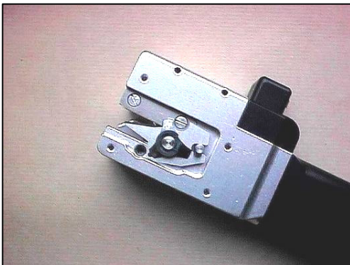
Figure 22. Knife assembly in splicer
