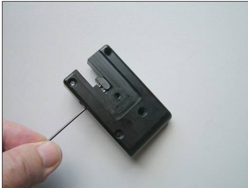
Figure 44. Remove yarn clamp stabilising pin securing screws
