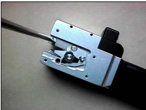
Figure 23. Knife assembly removal
