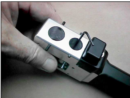
Figure 30. Unlock knife drive shaft
