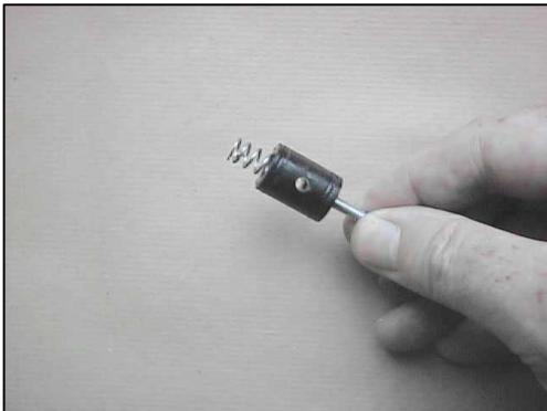
Figure 33. Knife drive piston assembly
