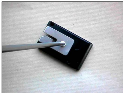
Figure 20. The simple splicer side-cheek - remove yarn guide plate exit side
