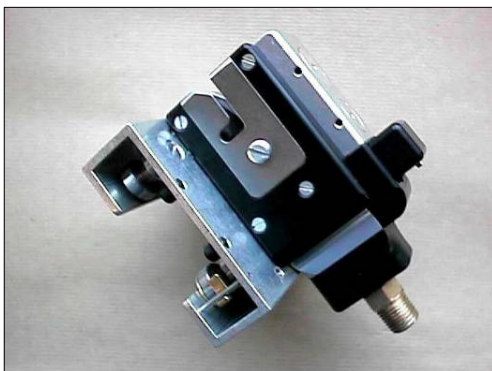
Figure 8. Model 103 B. Base unit without handle, close-fitted to a carriage running on a rail, simple side cheek
